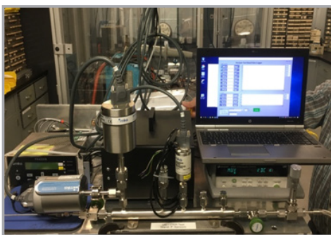
SVS pressure sensor electronics testing. Image: US ITER
