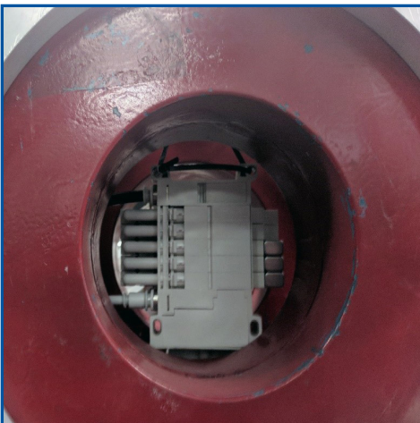
Solenoid valve manifold sandwiched between coil faces. Photo: US ITER/ORNL
